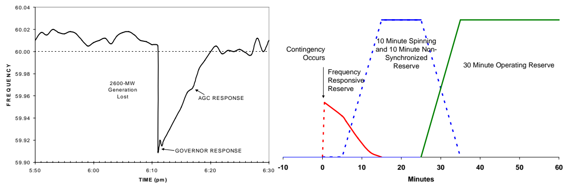
Figure 4 A series of contingency reserves are available to respond to the unexpected loss of a generator or transmission line.
