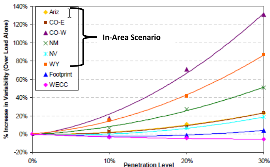
Figure 1. Percent Increase in Variability for In-Area Scenario – Western Wind and Solar Integration Study 206
