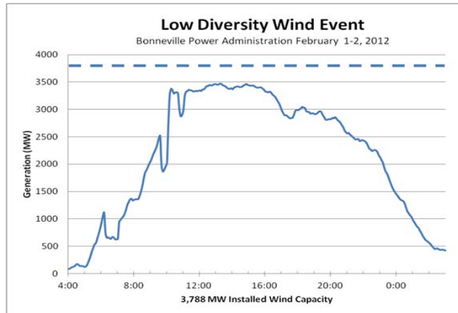
Figure 11. Recent Wind Event on BPA's System 247
