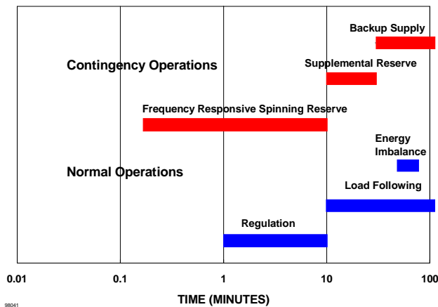
Fig. 1. Ancillary service dynamics.
